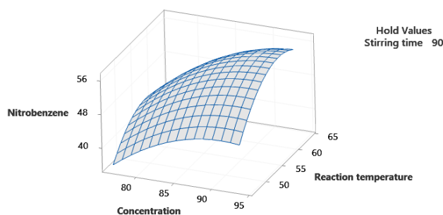
Fig. 10. Response results of nitrobenzene to sulfuric acid concentration on the silica ( X_1 ) and reaction temperature ( X_3 ) (a) contour plot and (b) response surface plot.
