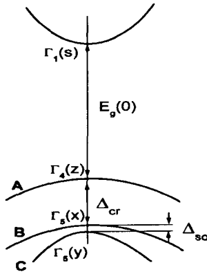
Fig. 5. Energy band structure of the chalcopyrite \text{AgInS}_2 at the \Gamma point according to the selection rule.
