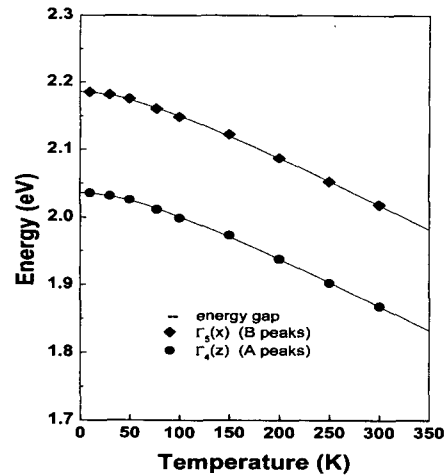
Fig. 4. Experimental values of the photocurrent peak energies and the energy band gap as a function of temperature.
