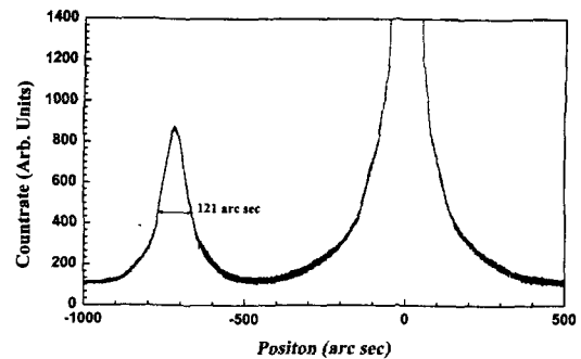
Fig. 2. X-ray double crystal rocking curves of the \text{AgInS}_2 epilayer.
