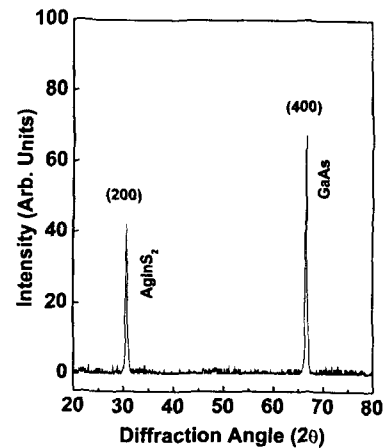
Fig. 1. X-ray diffraction patterns of the \text{AgInS}_2 epilayer grown on the GaAs substrate.
