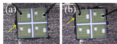
Fig. 6. Photographs of wetting flow of Sn-Sb BSM after die bonding (a) without and (b) with isothermal heat treatment.
